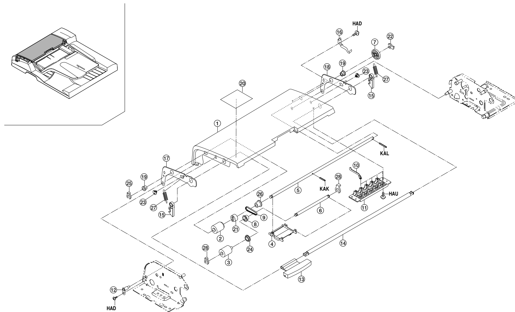
FIG. 2 PAPER FEED COVER
