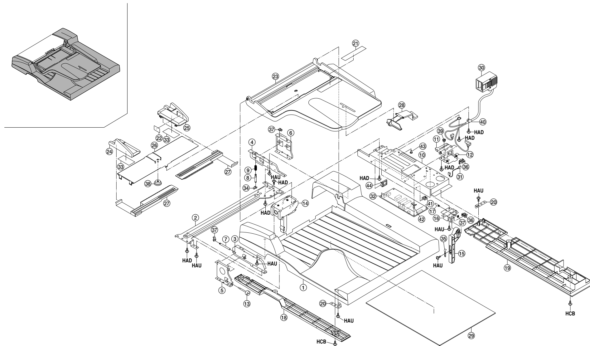
FIG. 1 HOUSING
